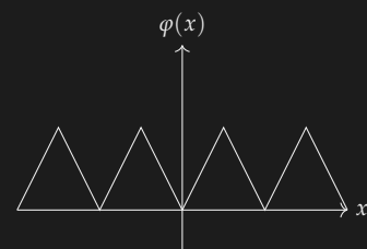
Figure 23.1: Sawtooth-like graph from \varphi
