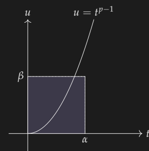
Figure 10.1: Motivation for Lemma 27.
