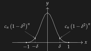
Figure 32.2: Dirac Sequence
