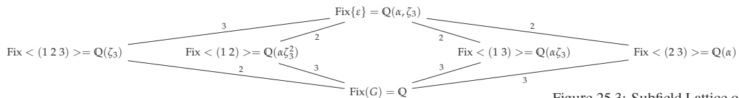
Figure 25.3: Subfield Lattice of \text{Gal}(\mathbb{Q}(\sqrt[3]{2}, \zeta_3)/\mathbb{Q})
