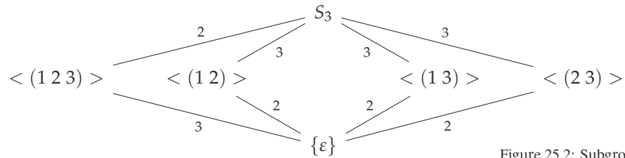
Figure 25.2: Subgroup Lattice of \text{Gal}(\mathbb{Q}(\sqrt[3]{2}, \zeta_3)/\mathbb{Q})
